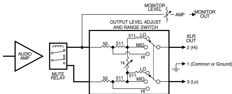
UCR300 Simplified Audio Output Circuit
