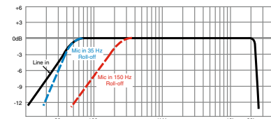
The roll-off slope steepens at lower frequencies.
